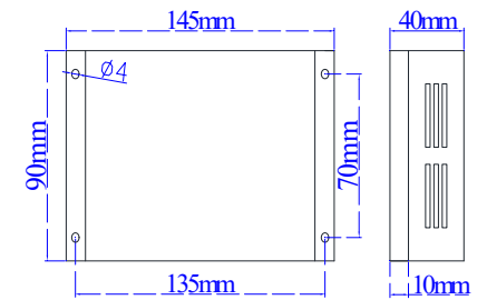
螺丝安装
